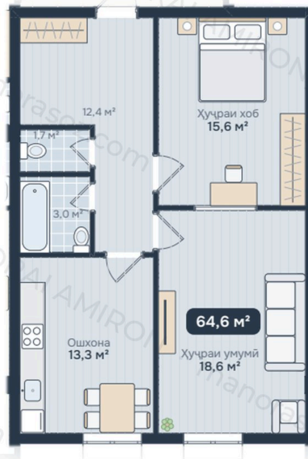
APARTMENT PLAN
